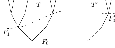
FIGURE 5. F_n is the front of n -th splitting nodes.
