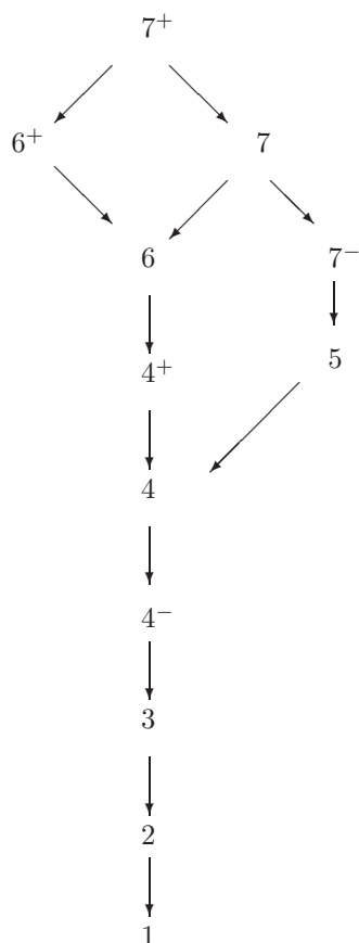
Implication Diagram
