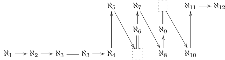
FIGURE 5. A possible assignment for Figure 2: \mathfrak{m} = \aleph_2 , \mathfrak{p} = \mathfrak{h} = \aleph_3 , \lambda_i = \aleph_{3+i} for i = 1, \dots, 9 . (Note that with the method of this section we cannot get \mathfrak{p} < \mathfrak{h} .)
