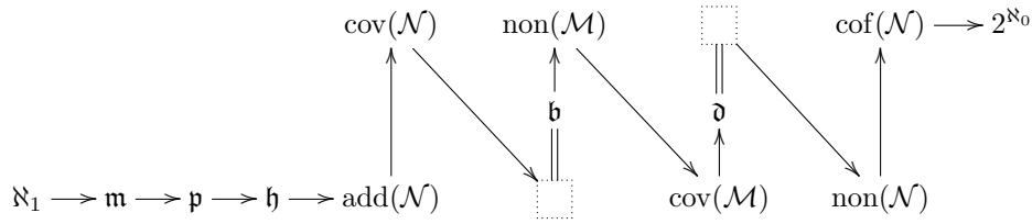
FIGURE 2. The model we construct in this paper; here \mathfrak{r} \rightarrow \mathfrak{q} means that \mathfrak{r} < \mathfrak{q} . When \mathfrak{h} is omitted, any number of the < signs can be replaced by = as desired (and in each such constellation we can get \mathfrak{p} = \mathfrak{h} ; see Remark 4.3 for details).
