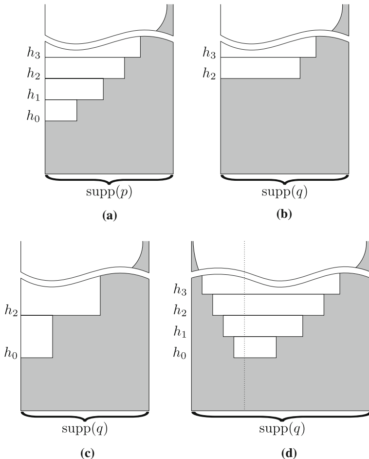
Fig. 3 a A schematic diagram of a condition p of the forcing. The h_i indicate an increasing enumeration of w^p , while the shaded region represents the domain of the trunk function t^p . b A condition q = p \wedge \eta , where \eta \in \text{poss}(p, < h_2) . In particular, all of the compound creatures above level h_2 have been left unchanged, and the level below h_2 the condition q consists entirely of trunk, with values determined by \eta . c A condition q obtained from p by gluing the pairs of compound creatures p(h_0), p(h_1) and p(h_2), p(h_3) . Note that \text{trklg}^q(\eta) = h_2 for any \eta \in \text{supp}(p) with \text{trklg}^p(\eta) = h_1 (and similarly if \text{trklg}^p(\eta) = h_3 ). d A condition q obtained as the “disjoint union” of p and another condition (represented to the left of the dotted line) with the same w and the same halving parameters at each level as p
