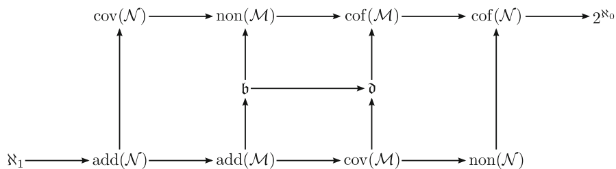
Fig. 1 Cichoń's diagram. An arrow between \mathfrak{r} and \mathfrak{\eta} indicates that \mathfrak{r} \leq \mathfrak{\eta} . Moreover, \max(\mathfrak{d}, \text{non}(\mathcal{M})) = \text{cof}(\mathcal{M}) and \min(\mathfrak{b}, \text{cov}(\mathcal{M})) = \text{add}(\mathcal{M})
