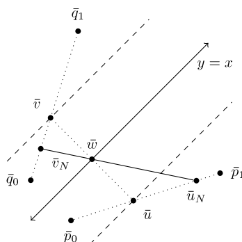
Fig. 3. The situation of Claim 5.6. The points \bar{u}_N and \bar{v}_N cannot be equidistant from \bar{w} , since one lies within the dashed parallel lines, and one lies without.
