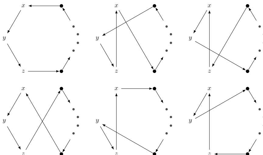
Fig. 1. Constructing a triangle from permutations of a cycle, as in Claim 4.5. Note that every edge is matched by an opposing one, except for xy , yz , and zx .
