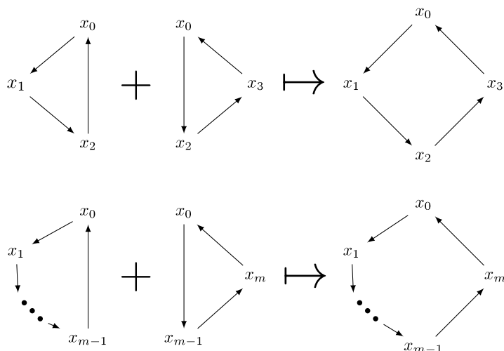
Fig. 2. Constructing a cycle from triangles, as in Claim 4.6.
