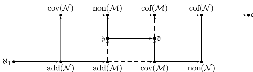
FIGURE 1. Cichoń's diagram
