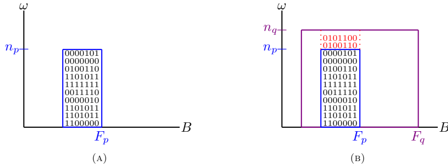
FIGURE 6. A condition p \in \mathbb{G}_{\mathbf{B}} is a binary function as in (A), whose domain is a finite square F_p \times n_p . The order is illustrated in (B): a condition q is stronger than p if q extends p and the new (horizontal) binary sequences between n_p and n_q respect \mathbf{B} \upharpoonright F_p .
