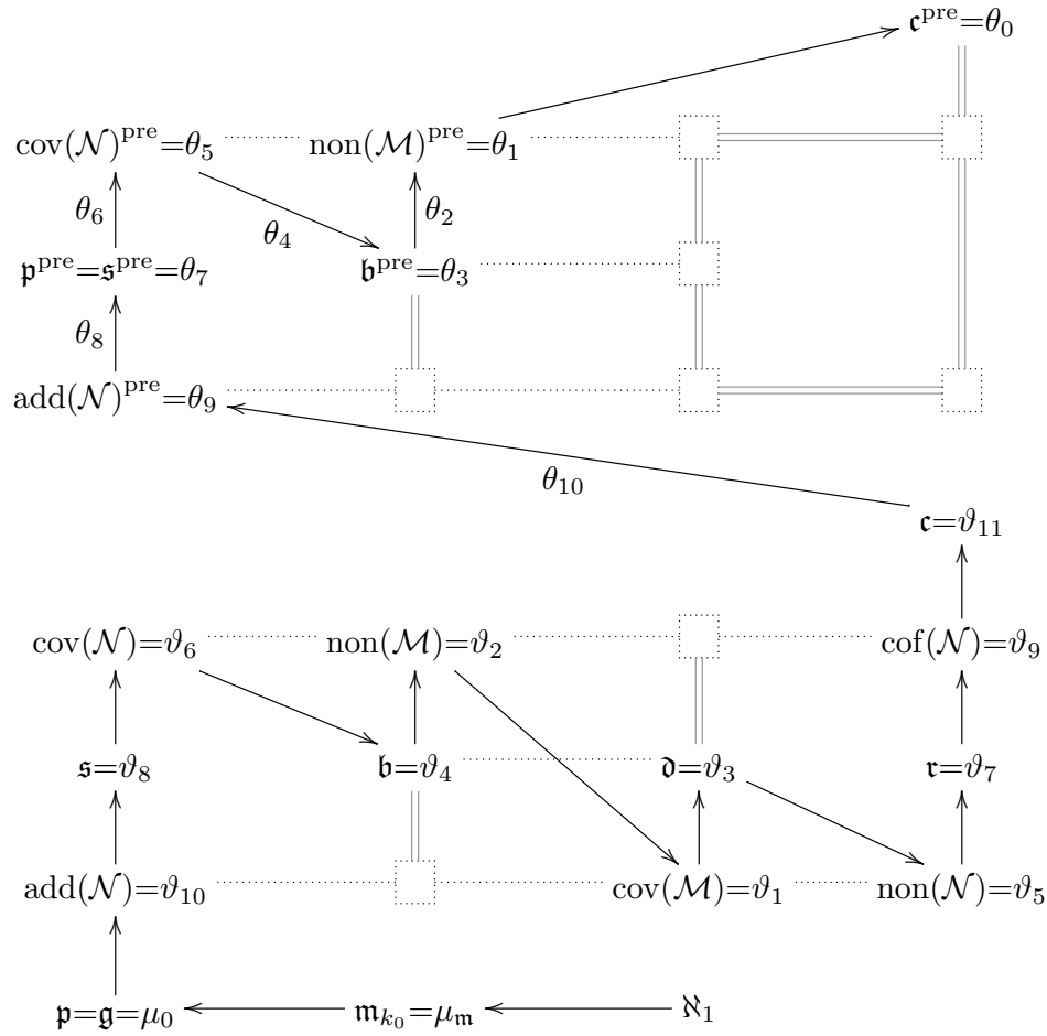
FIGURE 8. The cardinals \vartheta_n and \theta_n are increasing along the arrows. The upper diagram shows the situation forced by \mathbb{P}^0 , and the lower diagram shows the one forced by \mathbb{P}^1 . ( \mathfrak{s} can be anywhere between \mathfrak{p} and \mathfrak{b} .)
