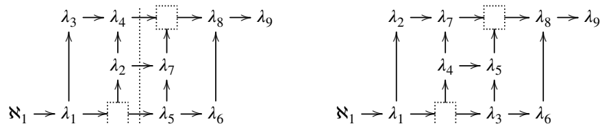
(A) An ordering compatible with FS ccc. (B) Another one, incompatible with FS ccc.
