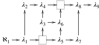
FIGURE 1. Our cardinal configuration (the \lambda_i are increasing).
