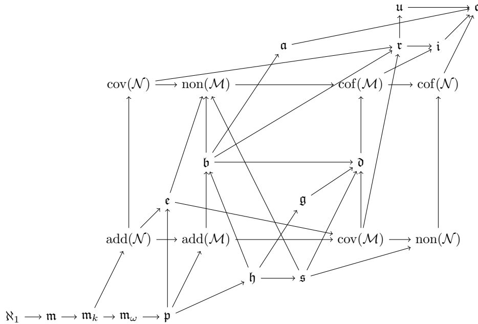
FIGURE 2. Cichoń's diagram and the Blass diagram combined. An arrow \mathfrak{r} \rightarrow \mathfrak{q} means that ZFC proves \mathfrak{r} \leq \mathfrak{q} .
