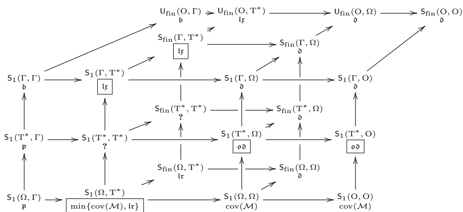
Fig. 1. The surviving properties
