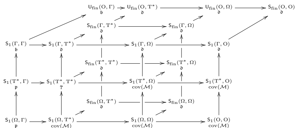
Fig. 2. The critical cardinalities in models of \mathfrak{c} \leq \aleph_2
