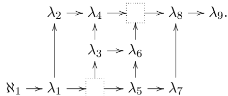
Figure 1. Our cardinal configuration. (The \lambda_i are increasing.)
